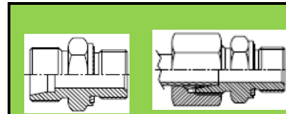
UNION MACHO BSPP C/JUNTA
