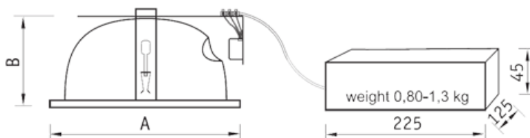
Luminaire with ECG.
